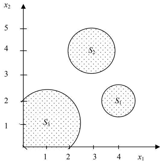
Figure 14. Feasible region of example 3.
