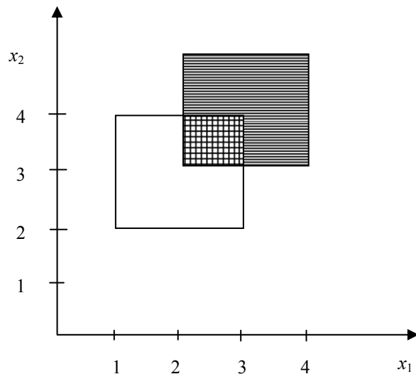
Figure 6. Intersecting disjunction.
