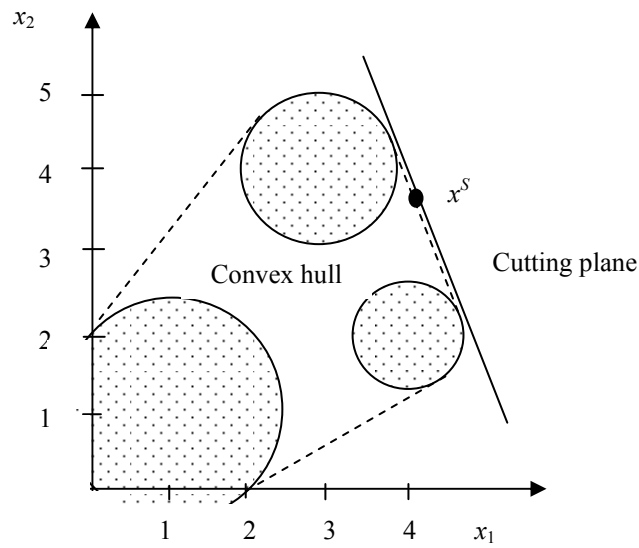
Figure 15. Convex hull and cutting plane for example 3.
