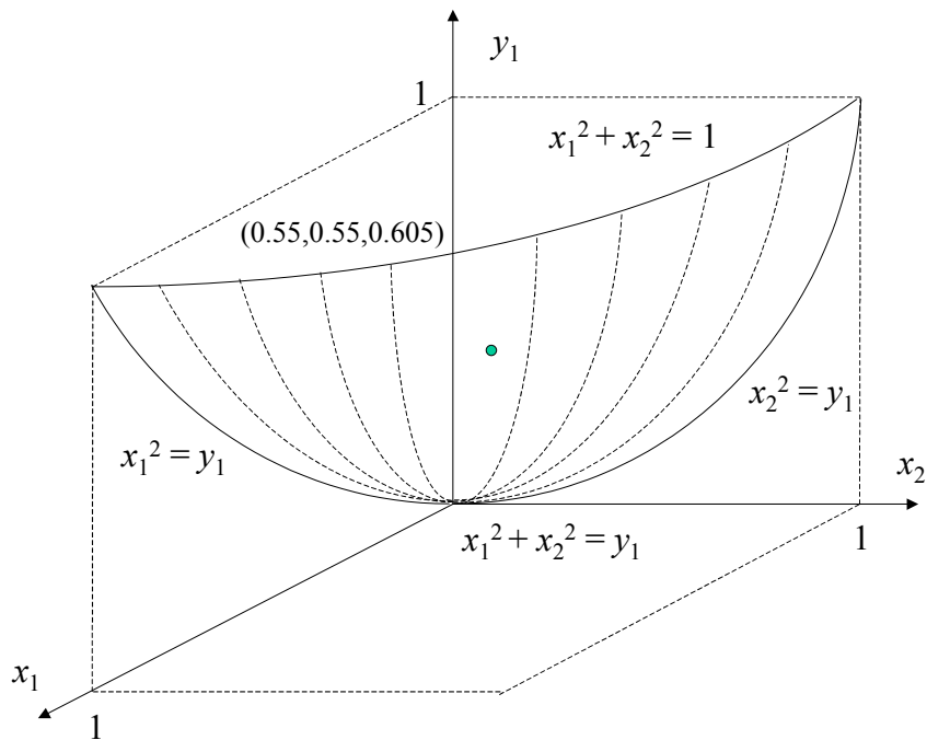
Figure 12. Big-M relaxation of example 2 in the x - y space.
