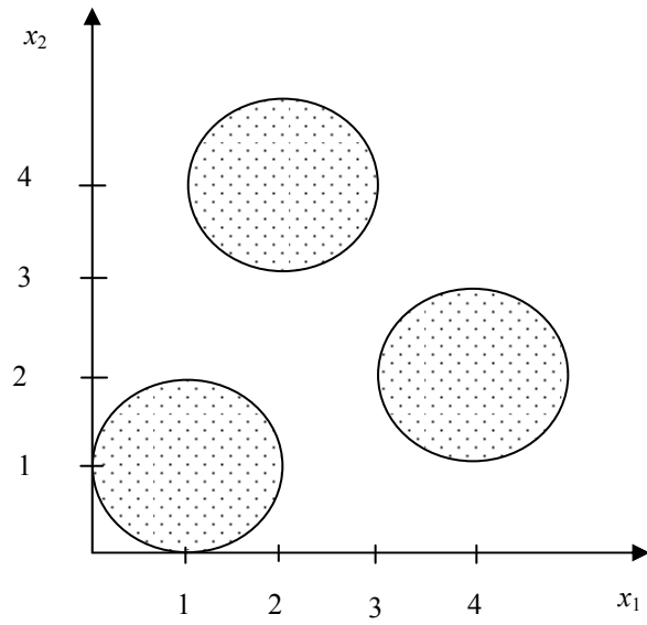
Figure 1. Feasible region of example 1.
