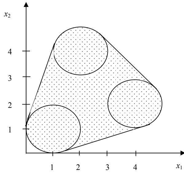
Figure 3. Convex hull relaxation of example 1.
