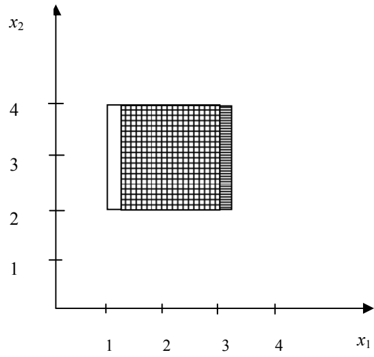
Figure 5. Intersecting disjunction.
