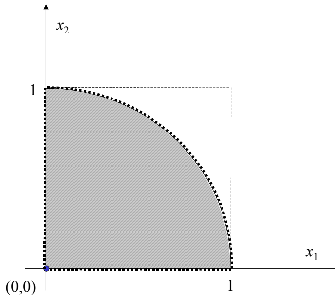
Figure 10. Feasible region of example 2 in the x space.
