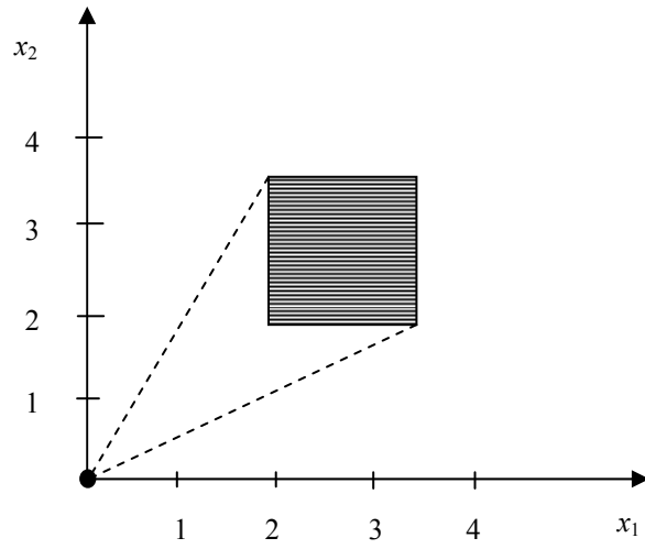
Figure 9. Disjoint disjunction with zero point.
