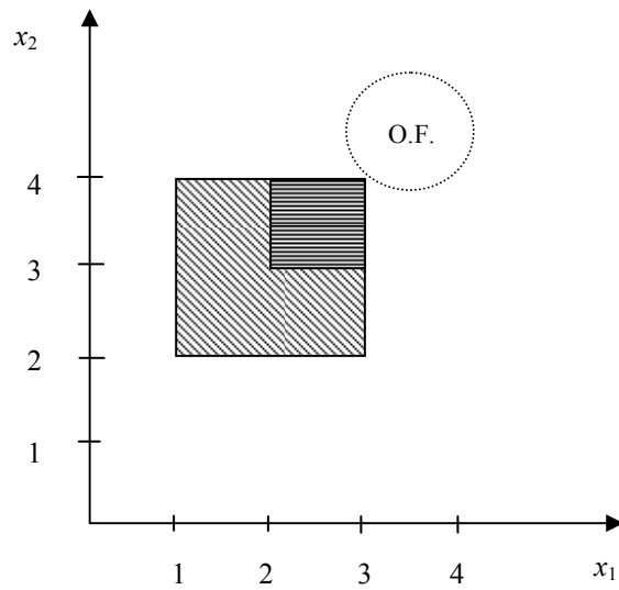
Figure 4. Feasible region of disjunctive set (20).
