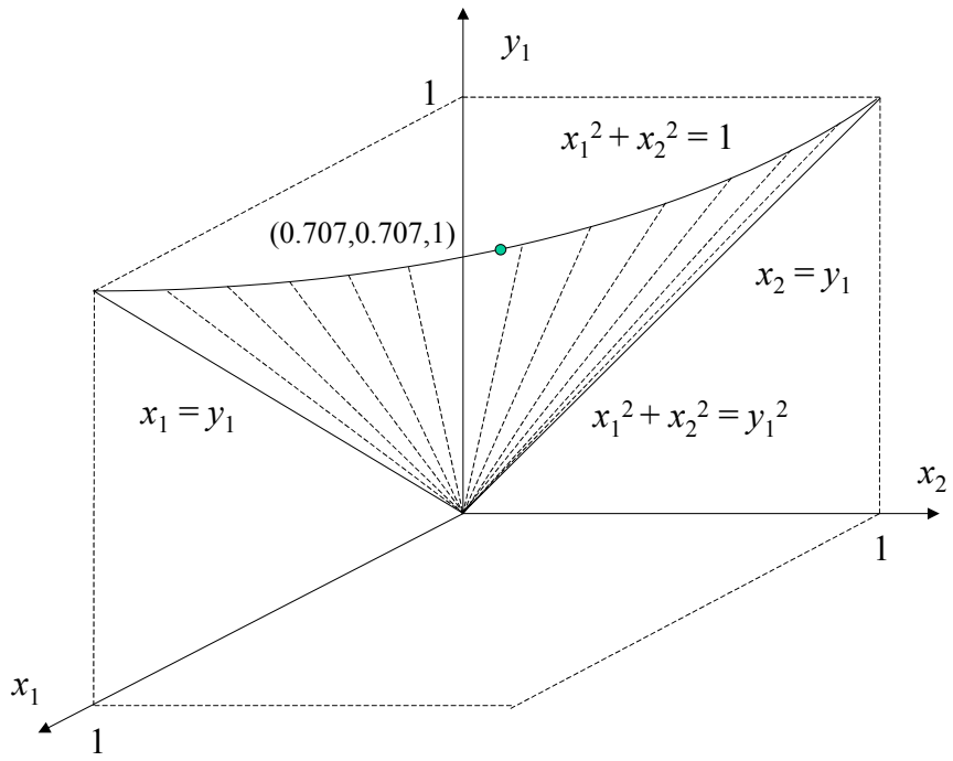
Figure 11. Convex hull relaxation of example 2 in the x - y space.
