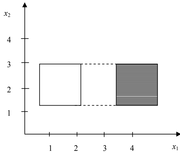
Figure 8. Disjoint disjunction (particular case).
