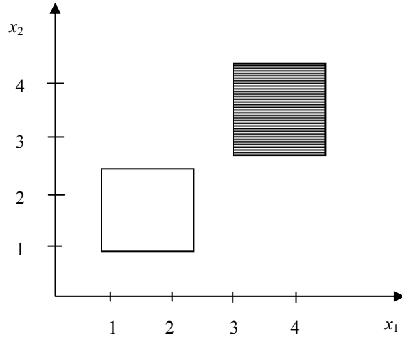
Figure 7. Disjoint disjunction (general case).
