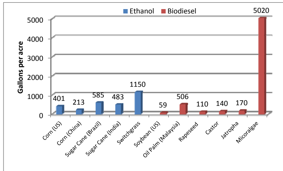
Figure 4.- Yield to ethanol and diesel form different raw materials 65-68
