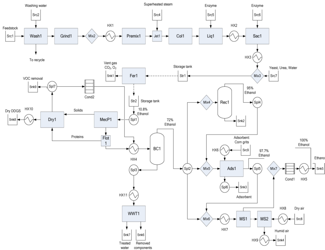
Figure 2.- Corn based ethanol production process
