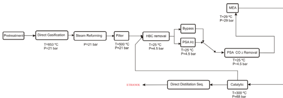
Figure 5. Thermo-chemical ethanol production from biomass
