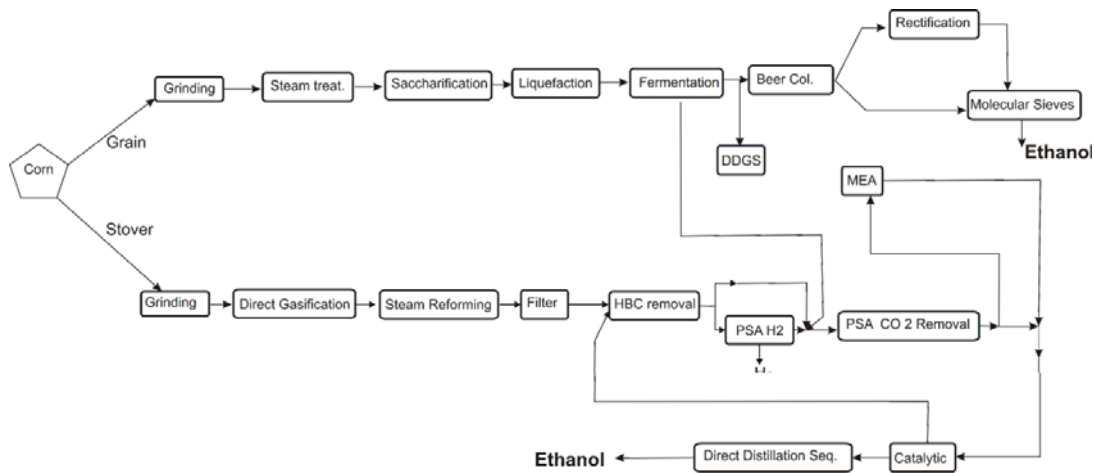
Figure 13.- Process integration for the simultaneous production of food and ethanol from corn
