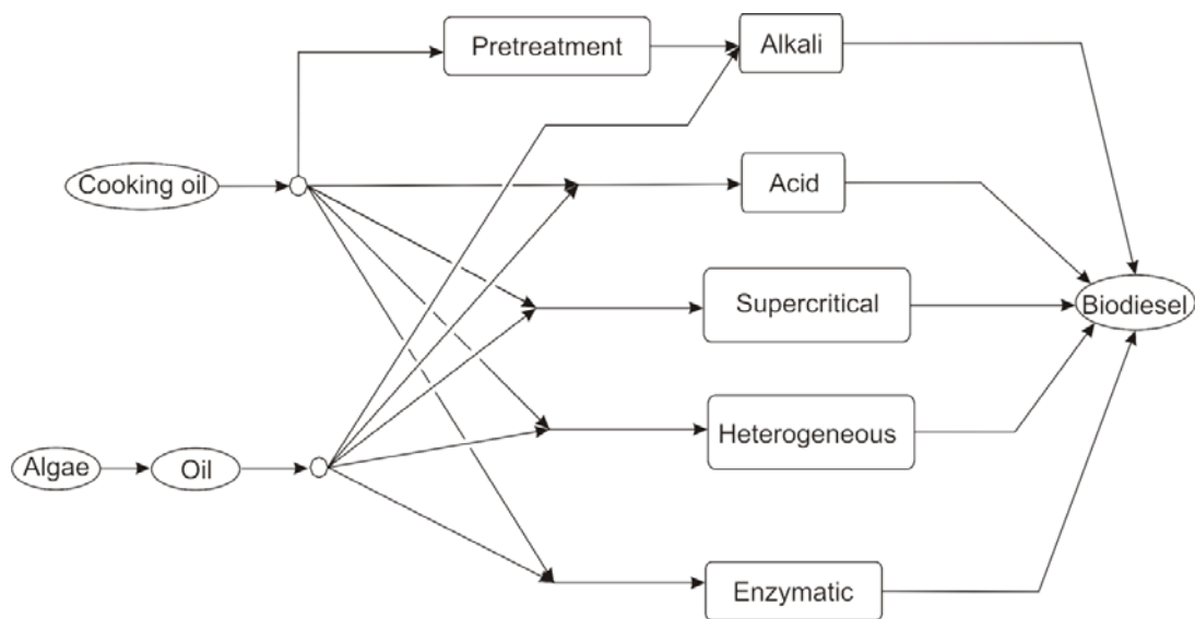
Figure 11.- Superstructure for the optimal production of biodiesel from oil
