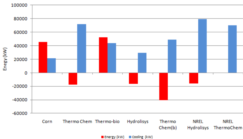
Figure 7.- Energy consumption and cooling needs for the ethanol production processes.
