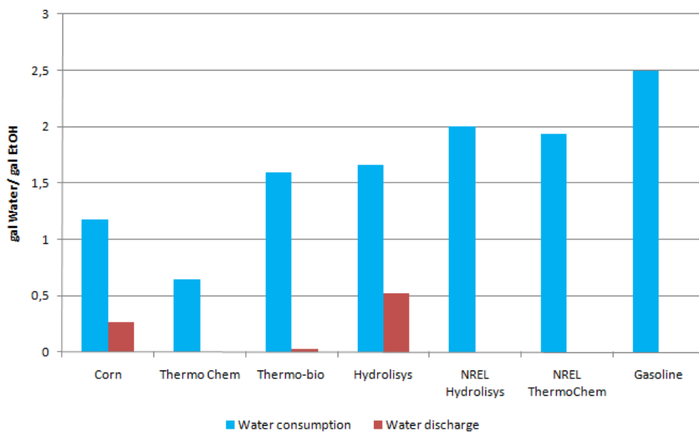
Figure 8.- Water consumption ethanol production processes.
