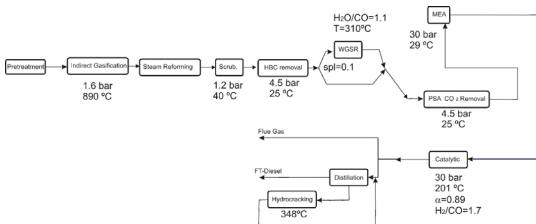
Figure 9.- Optimal flowsheet for the production of FT- Diesel.
