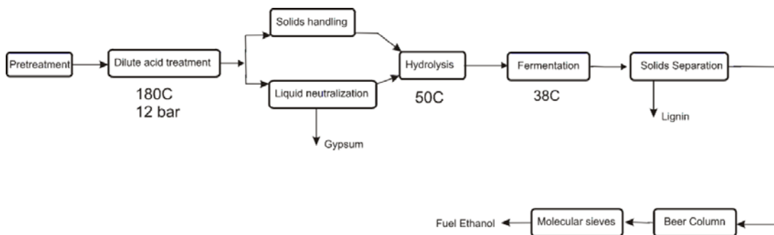
Figure 6.- Hydrolysis based production process of ethanol from switchgrass
