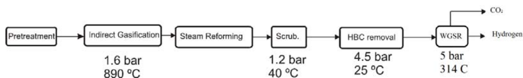
Figure 10.- Optimal flowsheet for the production of hydrogen from biomass
