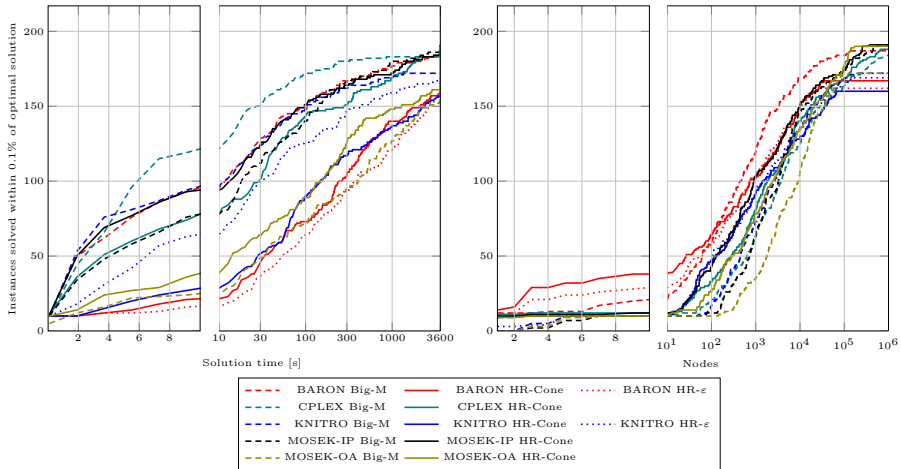
Fig. 1 Time (left) and nodes (right) performance profile for quadratic instances using the different GDP reformulations and commercial solvers.
