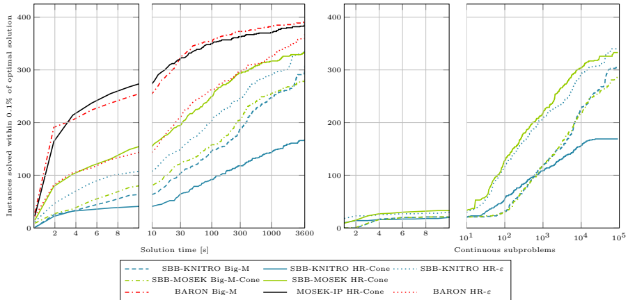
Fig. 3 Time (left) and Solved subproblems (right) performance profile for all instances using the different GDP reformulations and solvers through SBB. For the time profiles we include the best performing commercial solver results for each reformulation.
