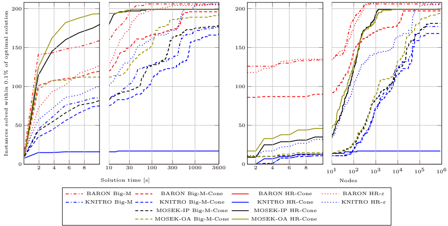
Fig. 2 Time (left) and Nodes (right) performance profile for exponential instances using the different GDP reformulations and commercial solvers.
